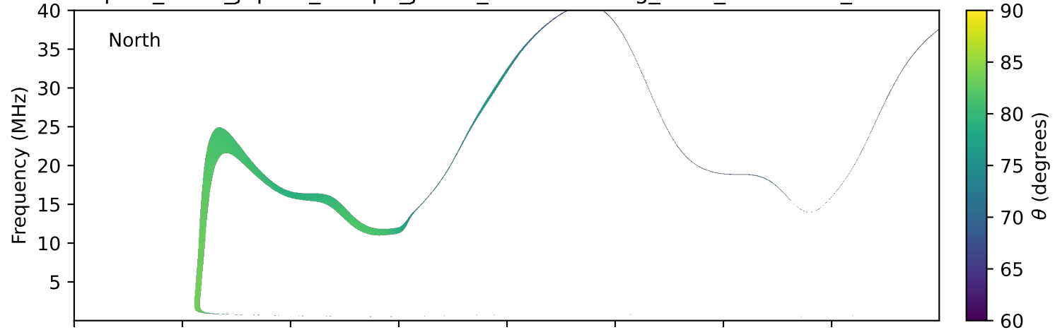
expres_earth_jupiter_europa_jrm33_lossc-wid1deg_3kev_20030218_v11.cdf
