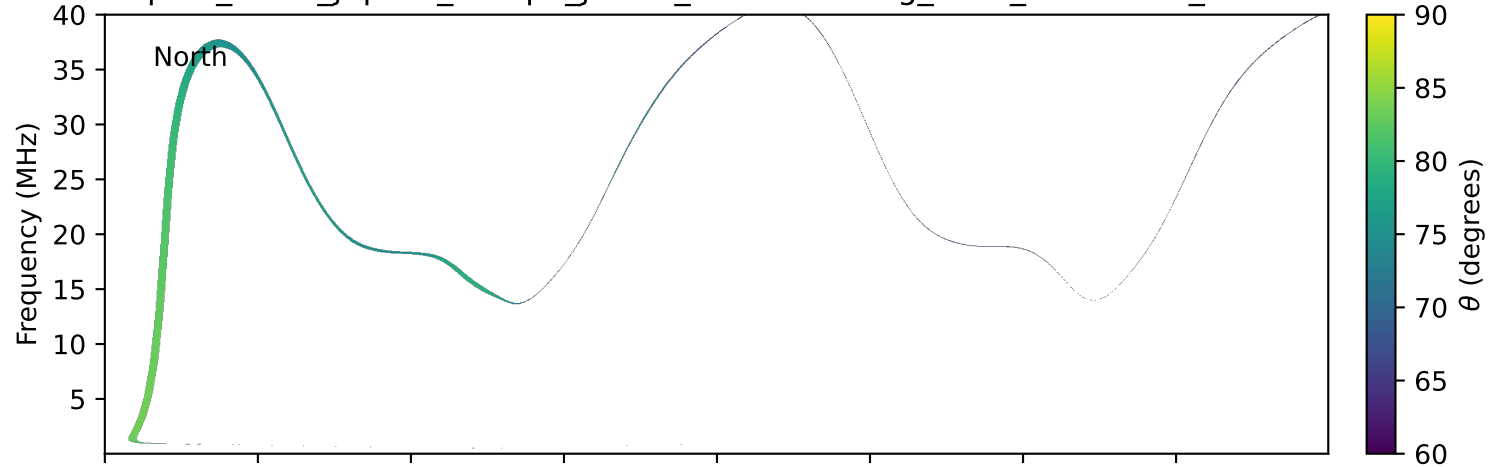
expres_earth_jupiter_europa_jrm33_lossc-wid1deg_3kev_20030204_v11.cdf
