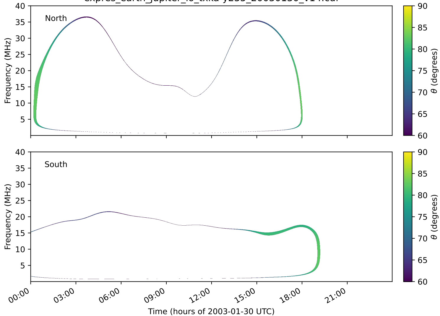
expres_earth_jupiter_io_txka-y235_20030130_v14.cdf
