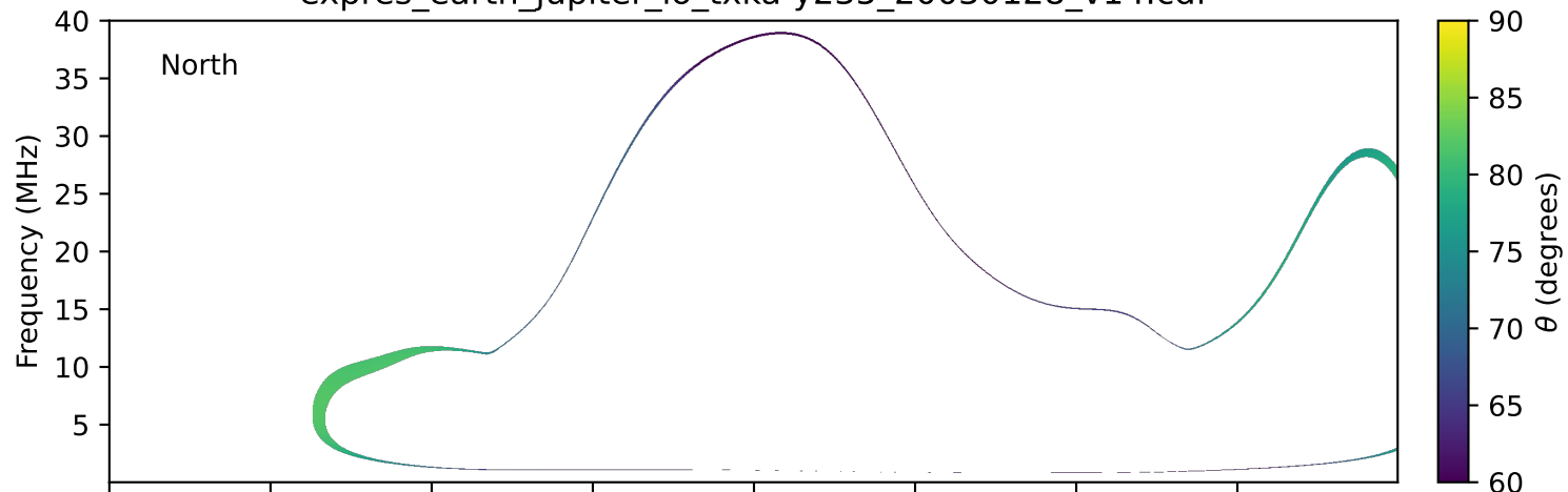
expres_earth_jupiter_io_txka-y235_20030128_v14.cdf
