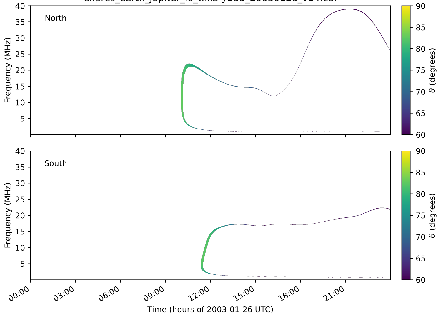
expres_earth_jupiter_io_txka-y235_20030126_v14.cdf
