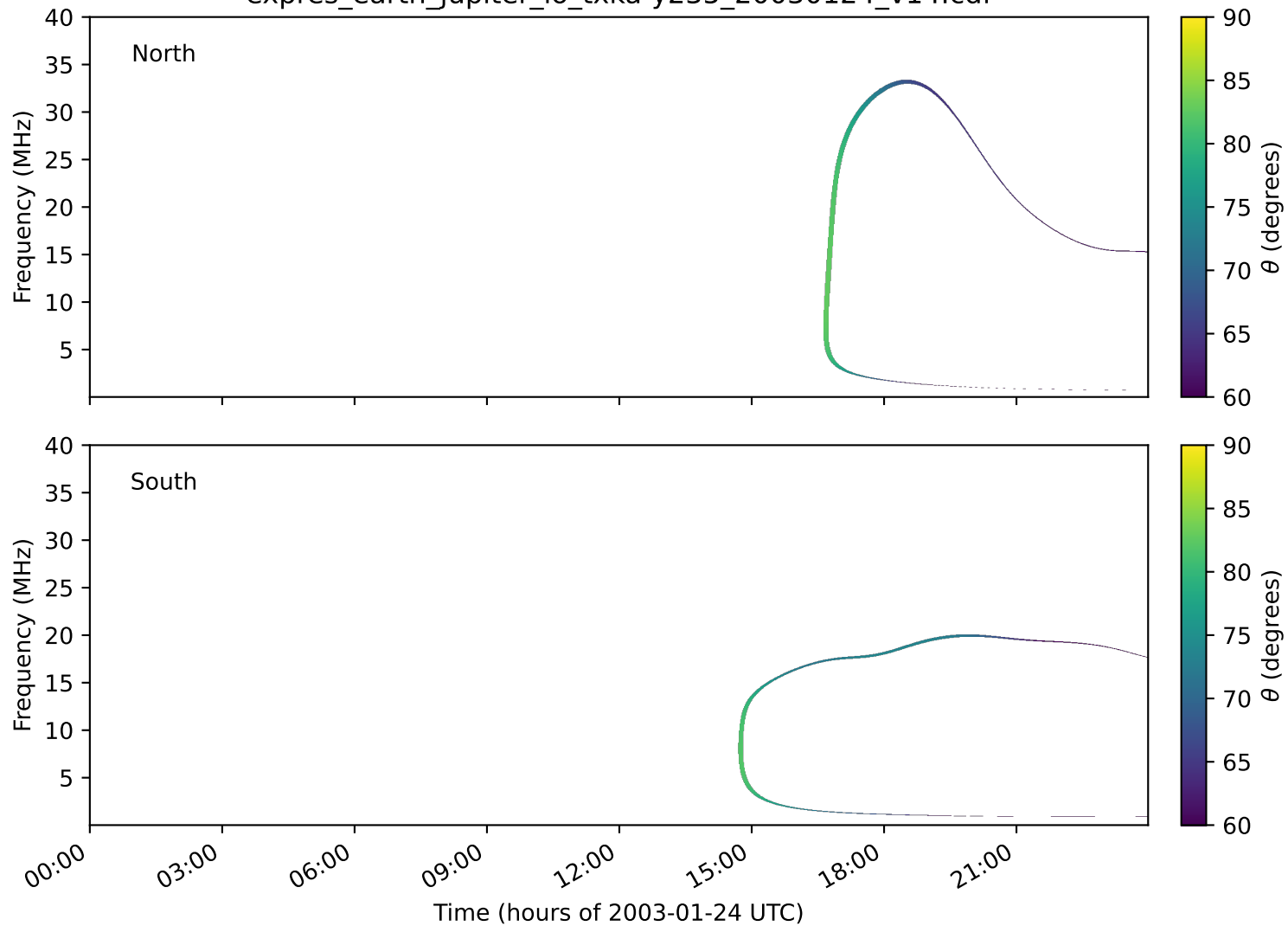
expres_earth_jupiter_io_txka-y235_20030124_v14.cdf
