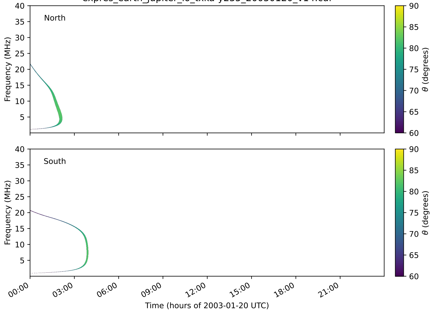
expres_earth_jupiter_io_txka-y235_20030120_v14.cdf
