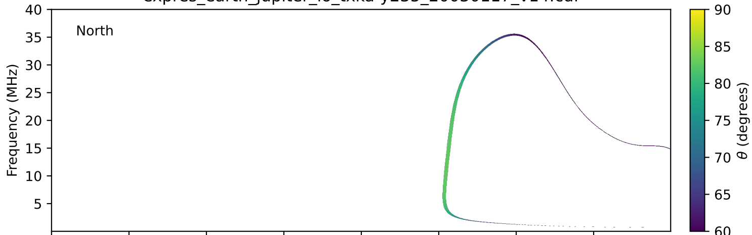
expres_earth_jupiter_io_txka-y235_20030117_v14.cdf
