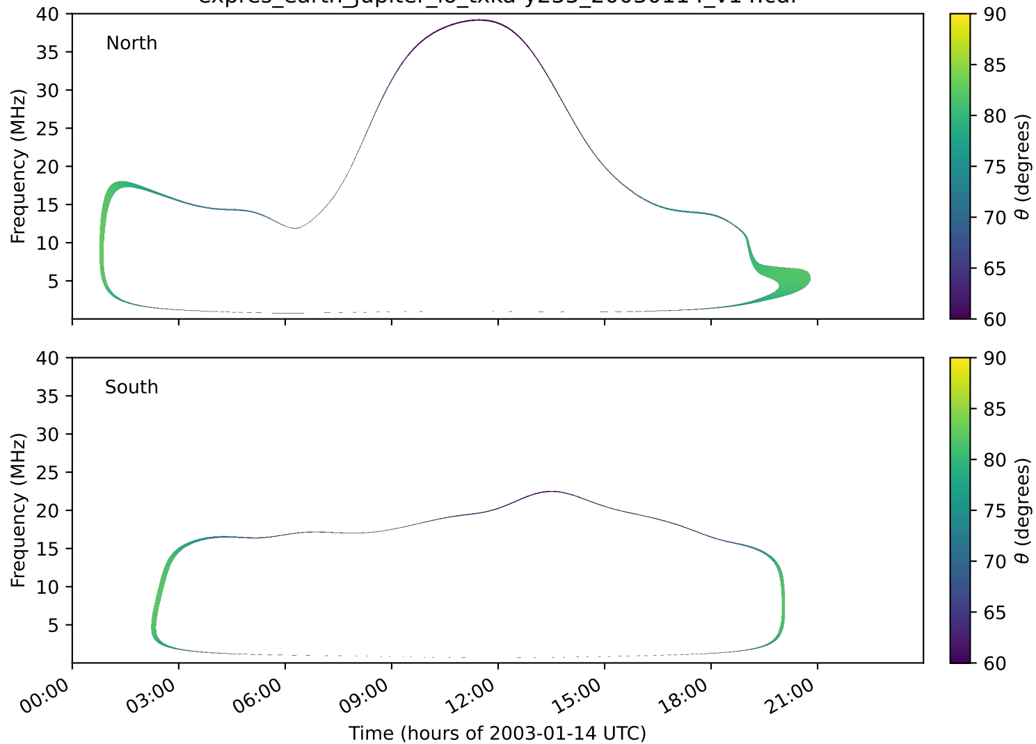
expres_earth_jupiter_io_txka-y235_20030114_v14.cdf
