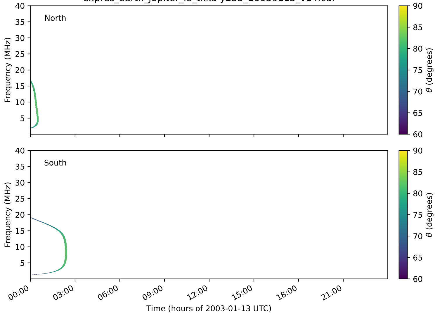
expres_earth_jupiter_io_txka-y235_20030113_v14.cdf
