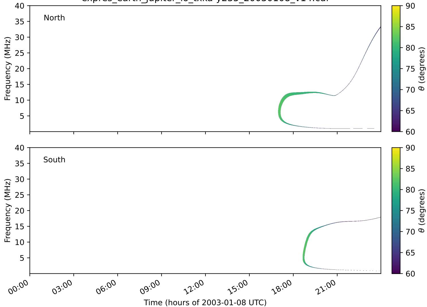
expres_earth_jupiter_io_txka-y235_20030108_v14.cdf
