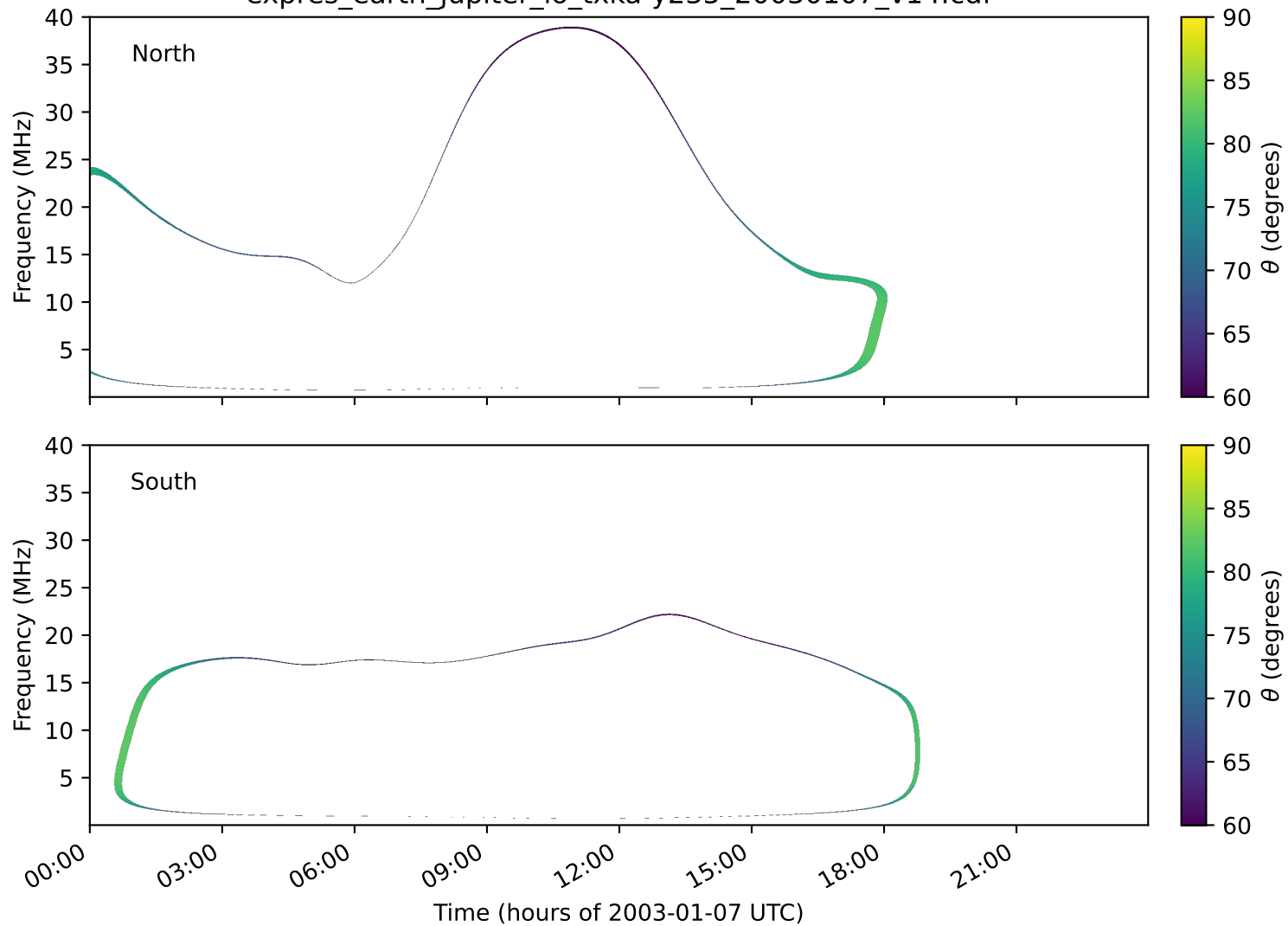
expres_earth_jupiter_io_txka-y235_20030107_v14.cdf
