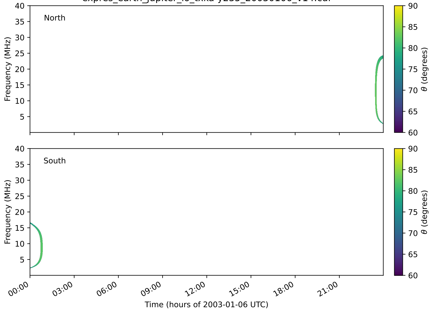
expres_earth_jupiter_io_txka-y235_20030106_v14.cdf
