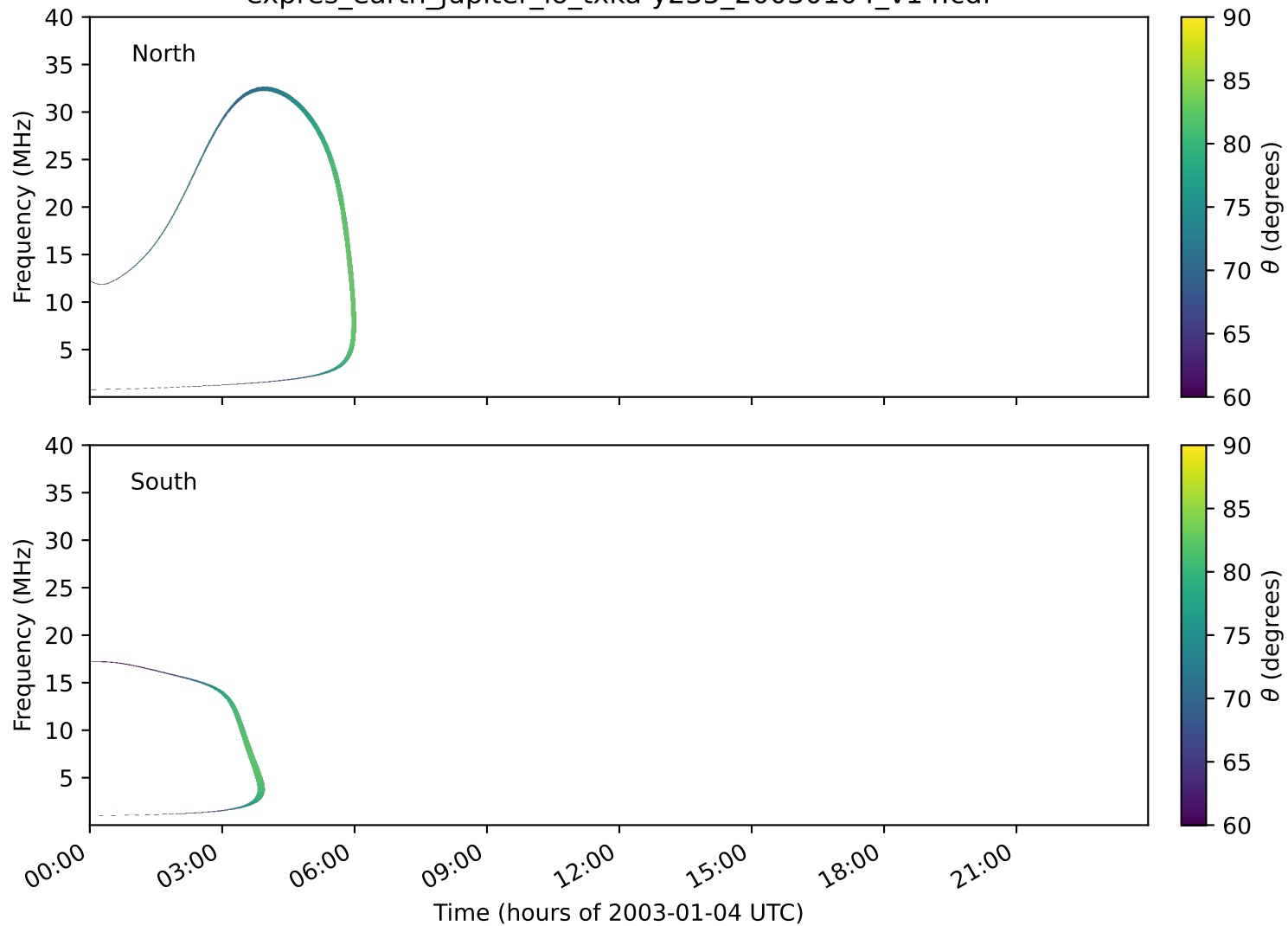
expres_earth_jupiter_io_txka-y235_20030104_v14.cdf
