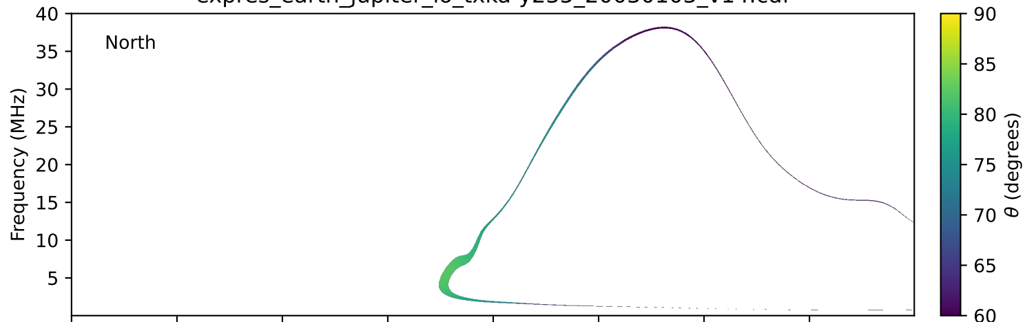
expres_earth_jupiter_io_txka-y235_20030103_v14.cdf
