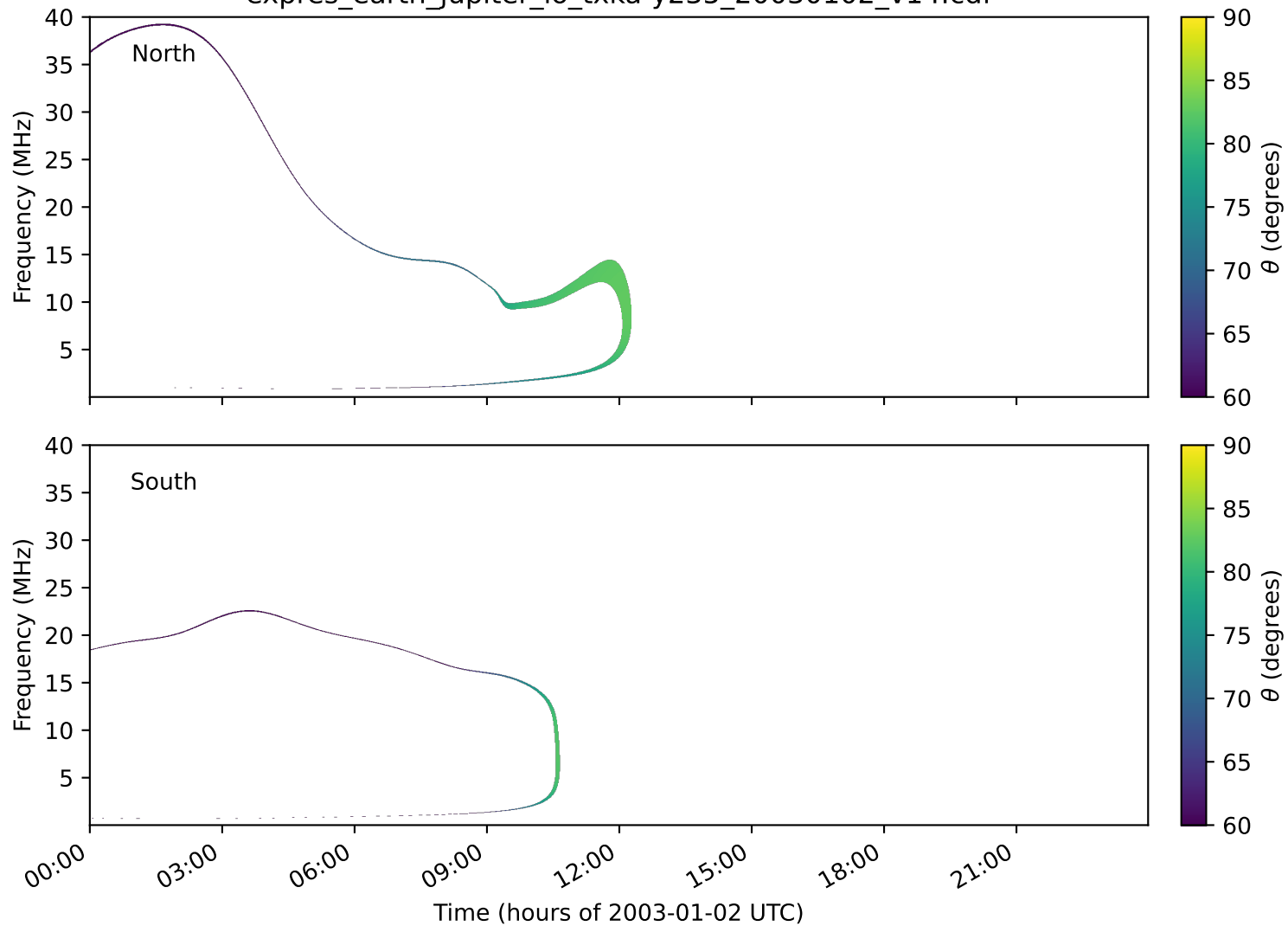
expres_earth_jupiter_io_txka-y235_20030102_v14.cdf
