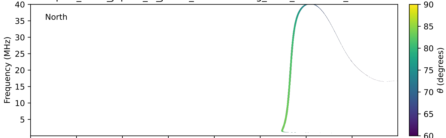
expres_earth_jupiter_io_jrm33_lossc-wid1deg_3kev_20030124_v11.cdf
