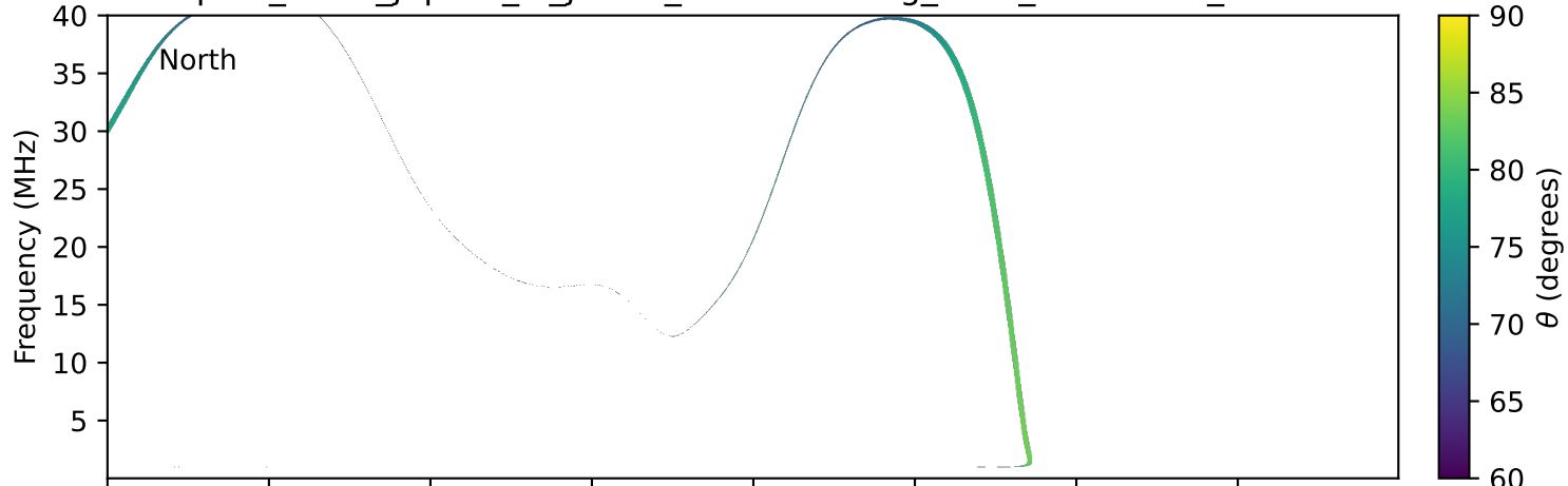
expres_earth_jupiter_io_jrm33_lossc-wid1deg_3kev_20030123_v11.cdf
