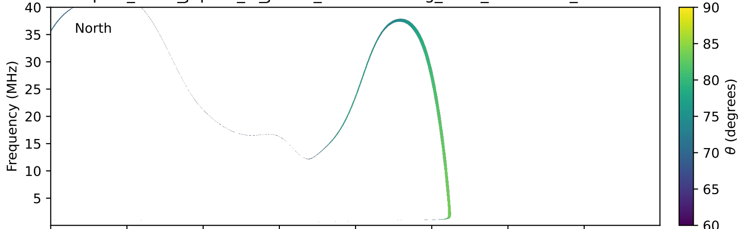
expres_earth_jupiter_io_jrm33_lossc-wid1deg_3kev_20030116_v11.cdf
