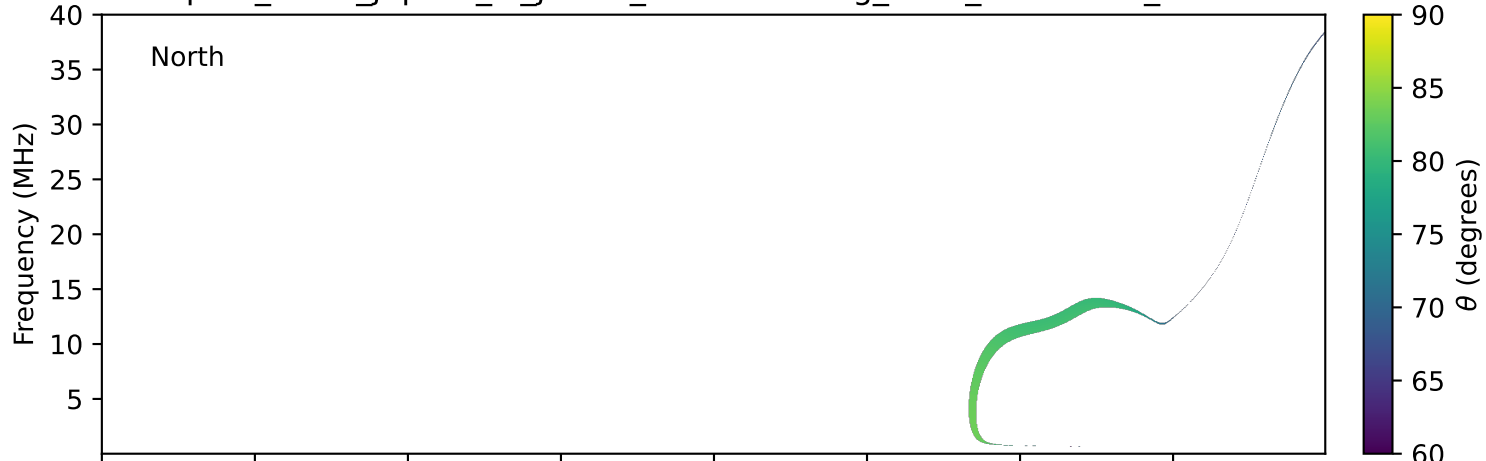
expres_earth_jupiter_io_jrm33_lossc-wid1deg_3kev_20030108_v11.cdf
