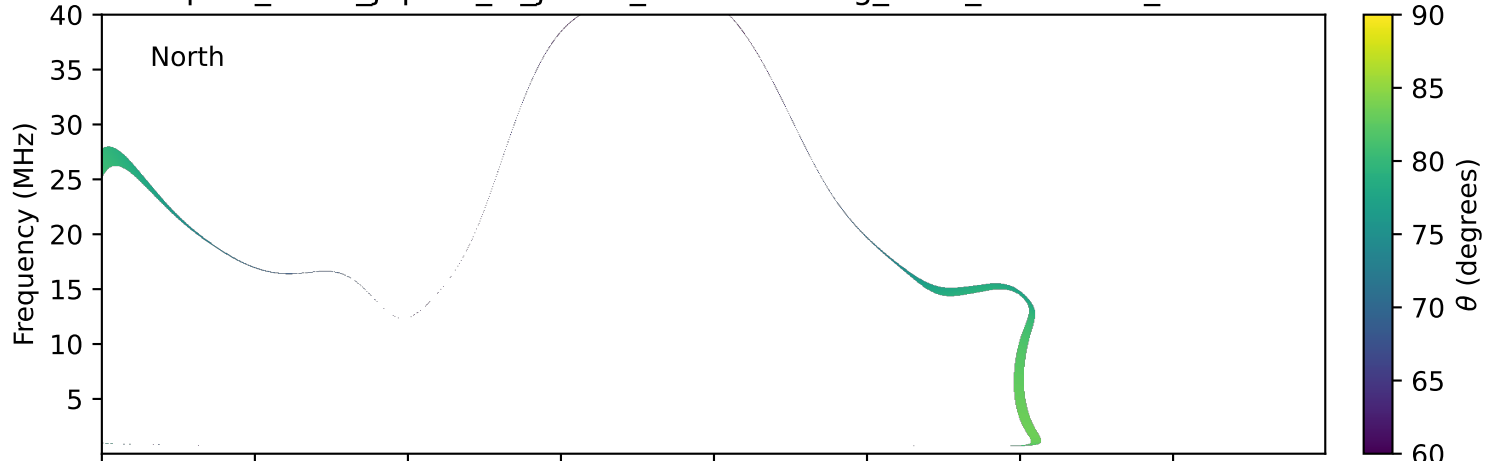
expres_earth_jupiter_io_jrm33_lossc-wid1deg_3kev_20030107_v11.cdf
