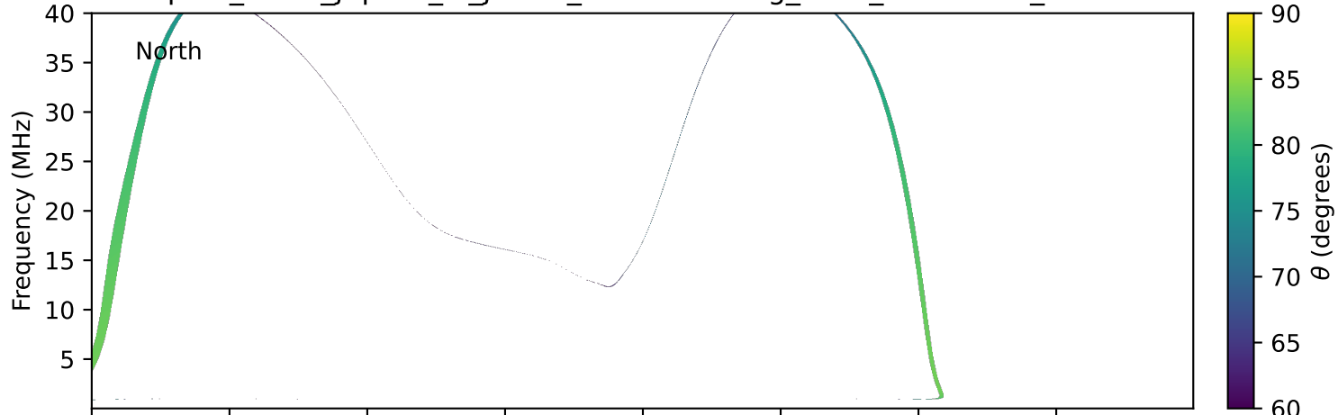
expres_earth_jupiter_io_jrm09_lossc-wid1deg_3kev_20030130_v11.cdf
