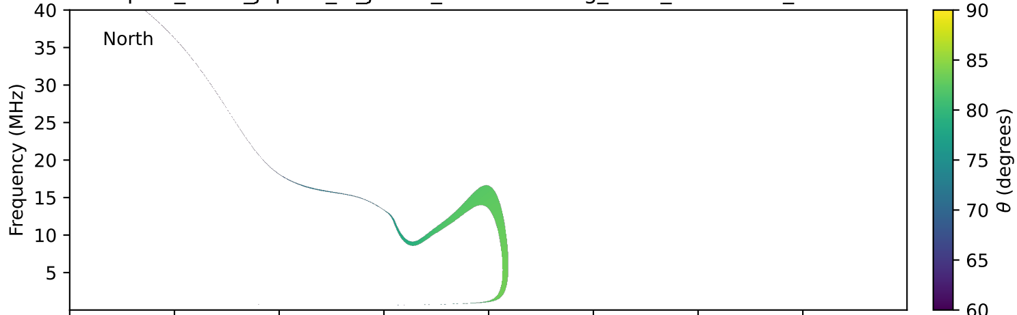
expres_earth_jupiter_io_jrm09_lossc-wid1deg_3kev_20030102_v11.cdf
