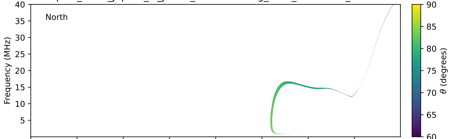
expres_earth_jupiter_io_jrm09_lossc-wid1deg_3kev_20030101_v11.cdf
