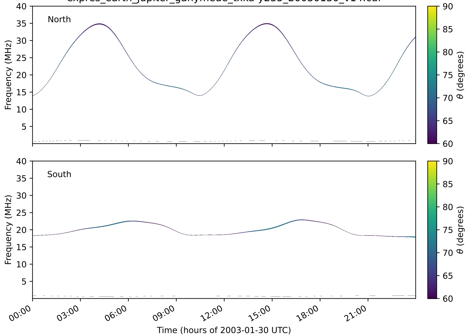
expres_earth_jupiter_ganymede_txka-y235_20030130_v14.cdf
