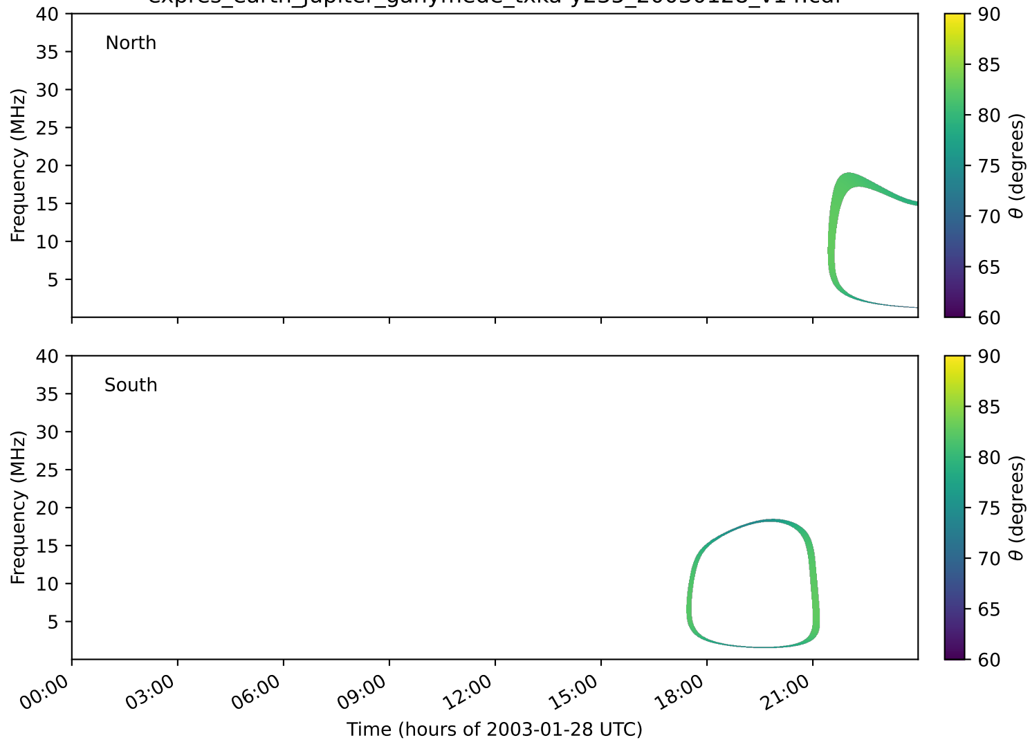
expres_earth_jupiter_ganymede_txka-y235_20030128_v14.cdf
