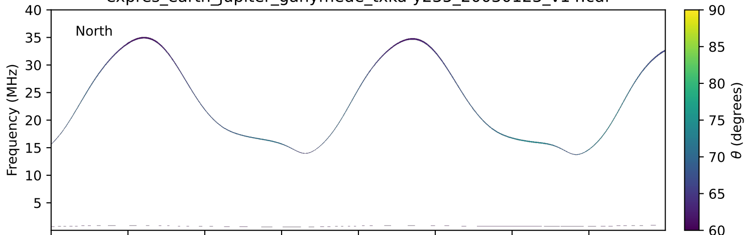
expres_earth_jupiter_ganymede_txka-y235_20030123_v14.cdf
