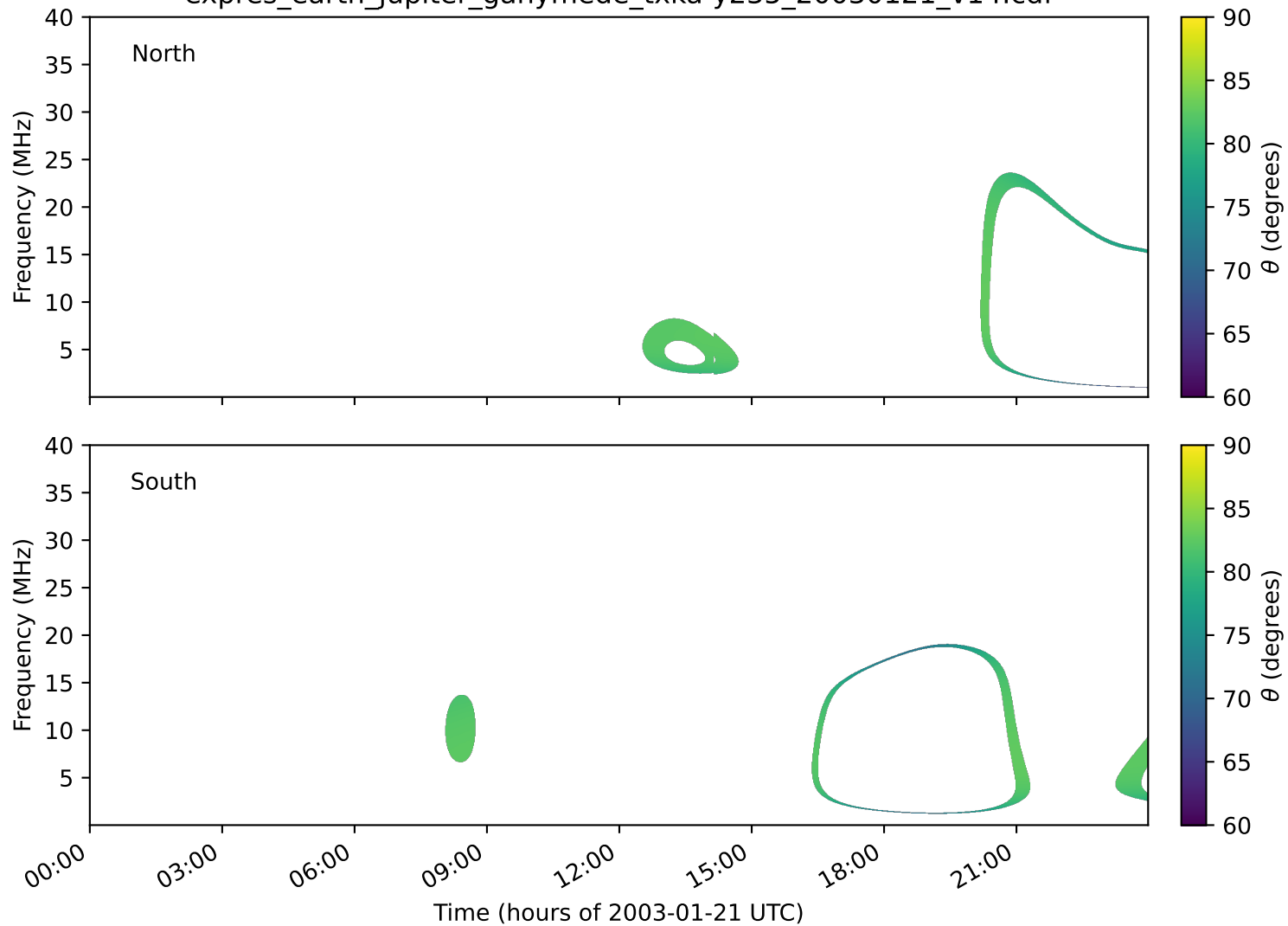
expres_earth_jupiter_ganymede_txka-y235_20030121_v14.cdf
