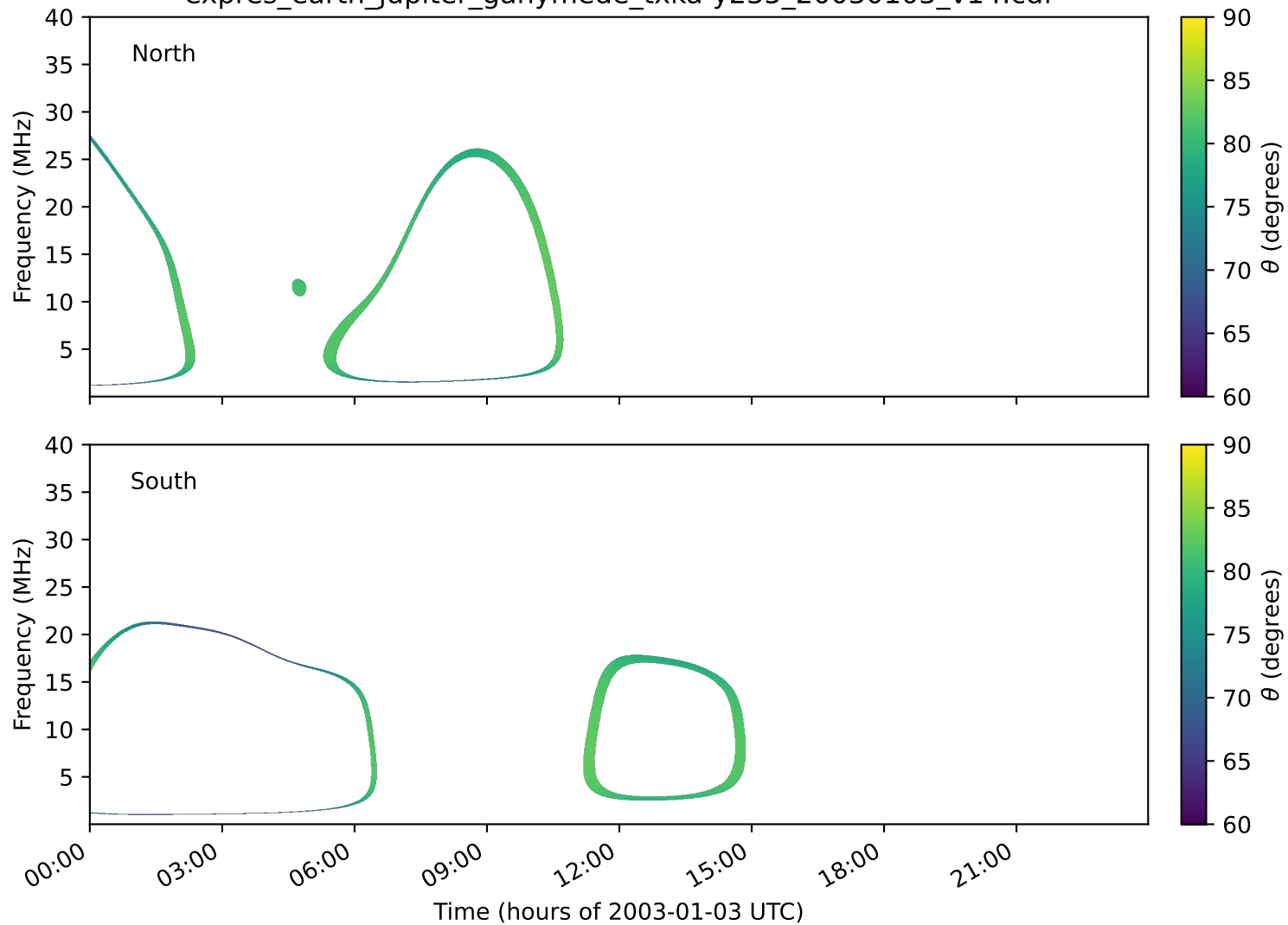
expres_earth_jupiter_ganymede_txka-y235_20030103_v14.cdf
