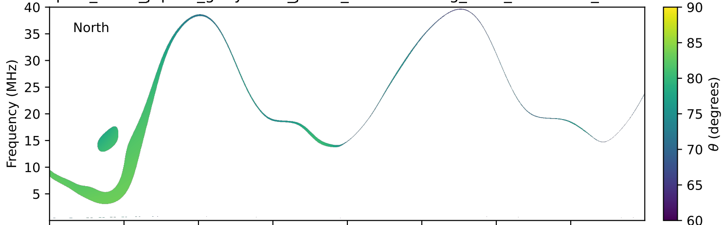
expres_earth_jupiter_ganymede_jrm33_lossc-wid1deg_3kev_20030115_v11.cdf
