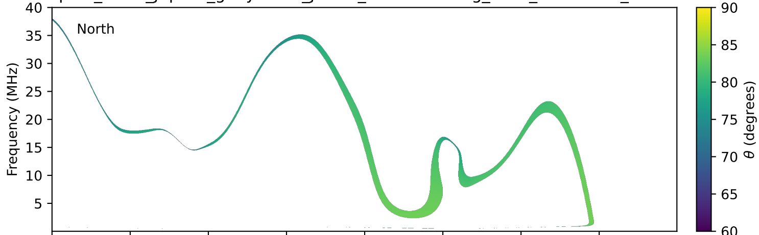
expres_earth_jupiter_ganymede_jrm33_lossc-wid1deg_3kev_20030110_v11.cdf
