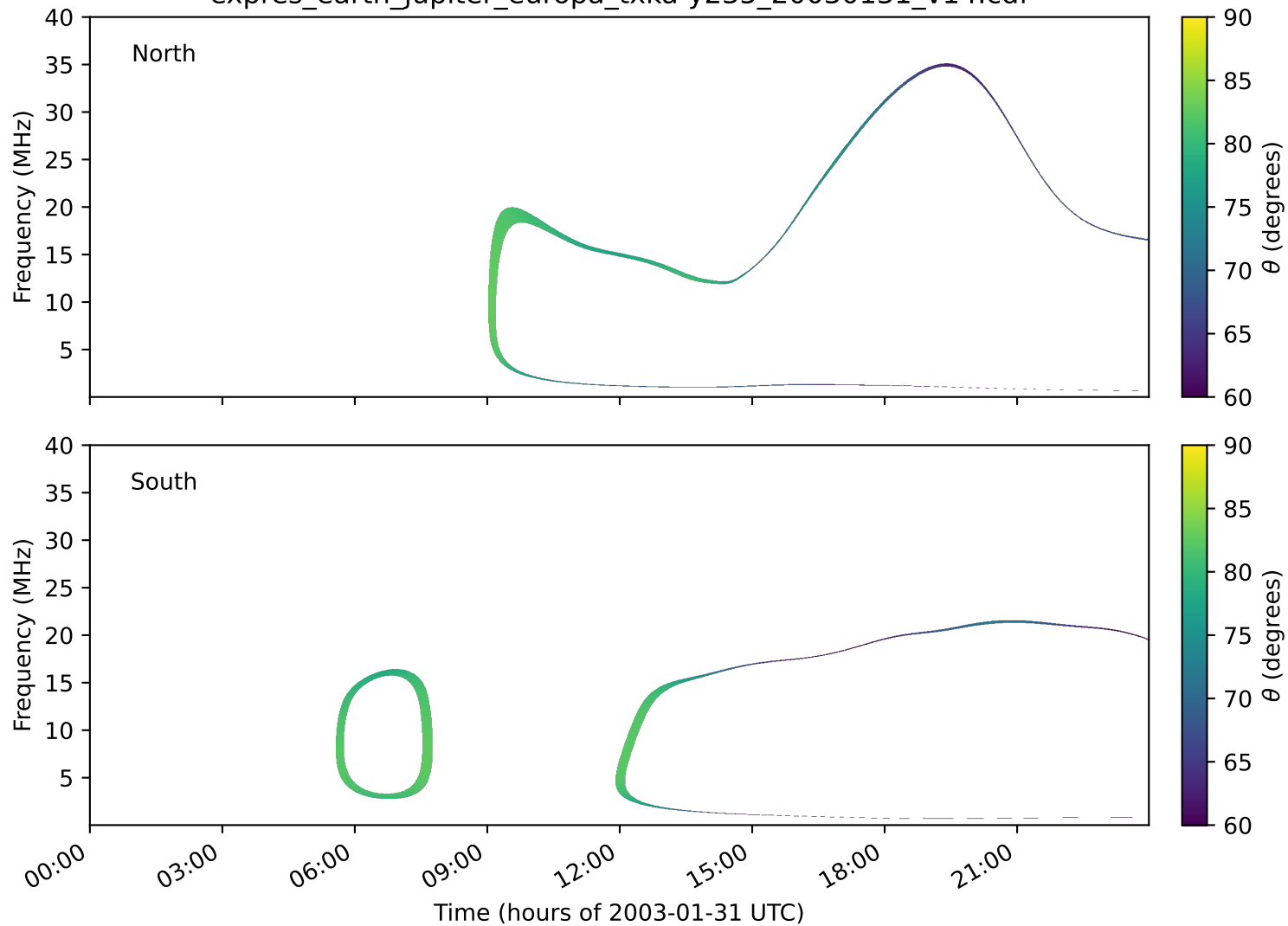
expres_earth_jupiter_europa_txka-y235_20030131_v14.cdf
