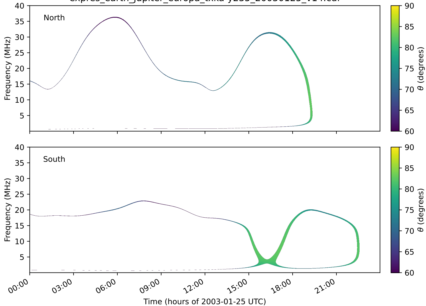
expres_earth_jupiter_europa_txka-y235_20030125_v14.cdf
