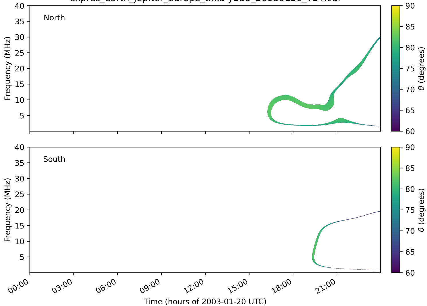
expres_earth_jupiter_europa_txka-y235_20030120_v14.cdf
