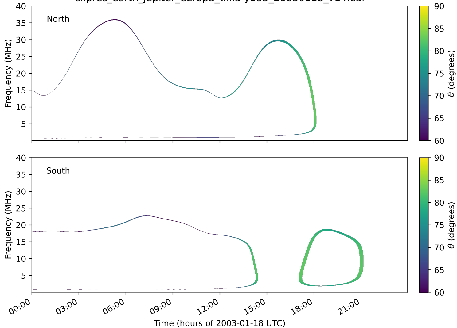
expres_earth_jupiter_europa_txka-y235_20030118_v14.cdf
