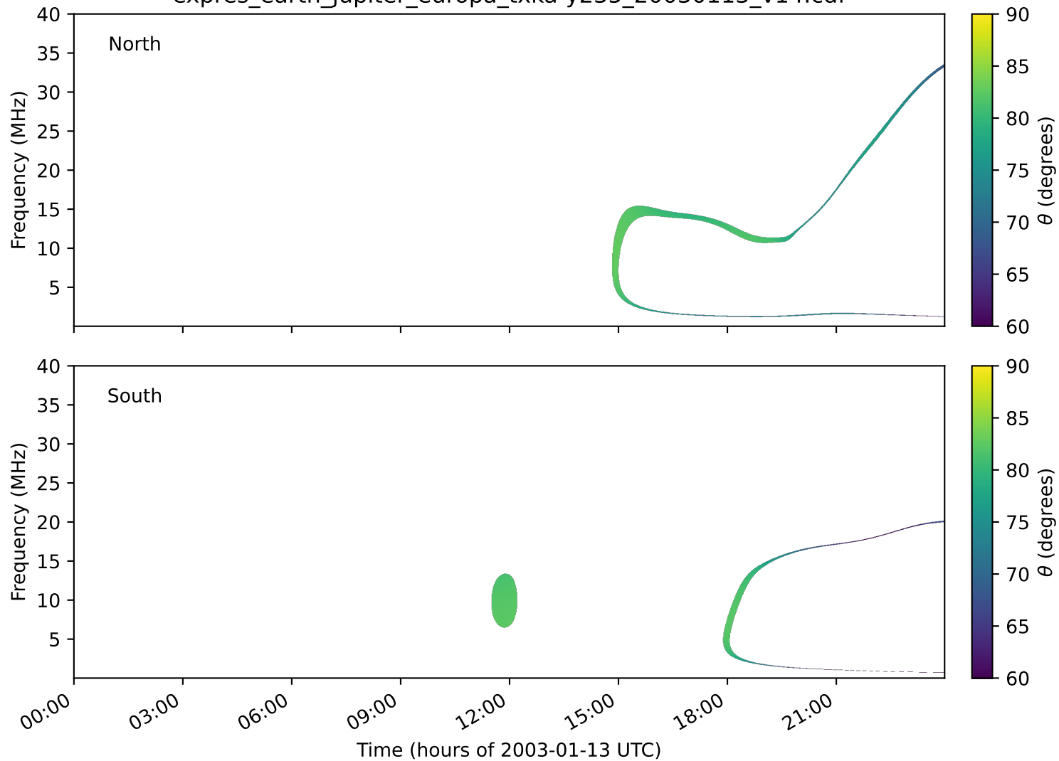
expres_earth_jupiter_europa_txka-y235_20030113_v14.cdf
