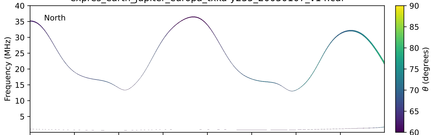
expres_earth_jupiter_europa_txka-y235_20030107_v14.cdf
