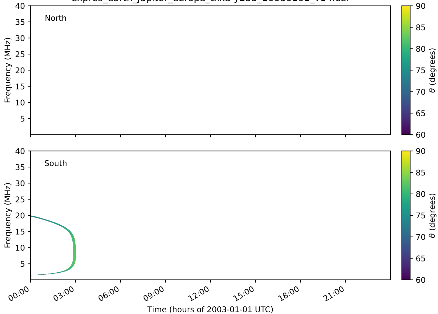
expres_earth_jupiter_europa_txka-y235_20030101_v14.cdf
