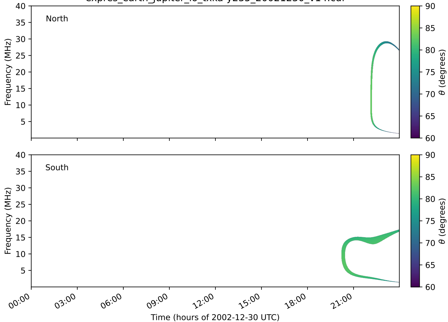
expres_earth_jupiter_io_txka-y235_20021230_v14.cdf
