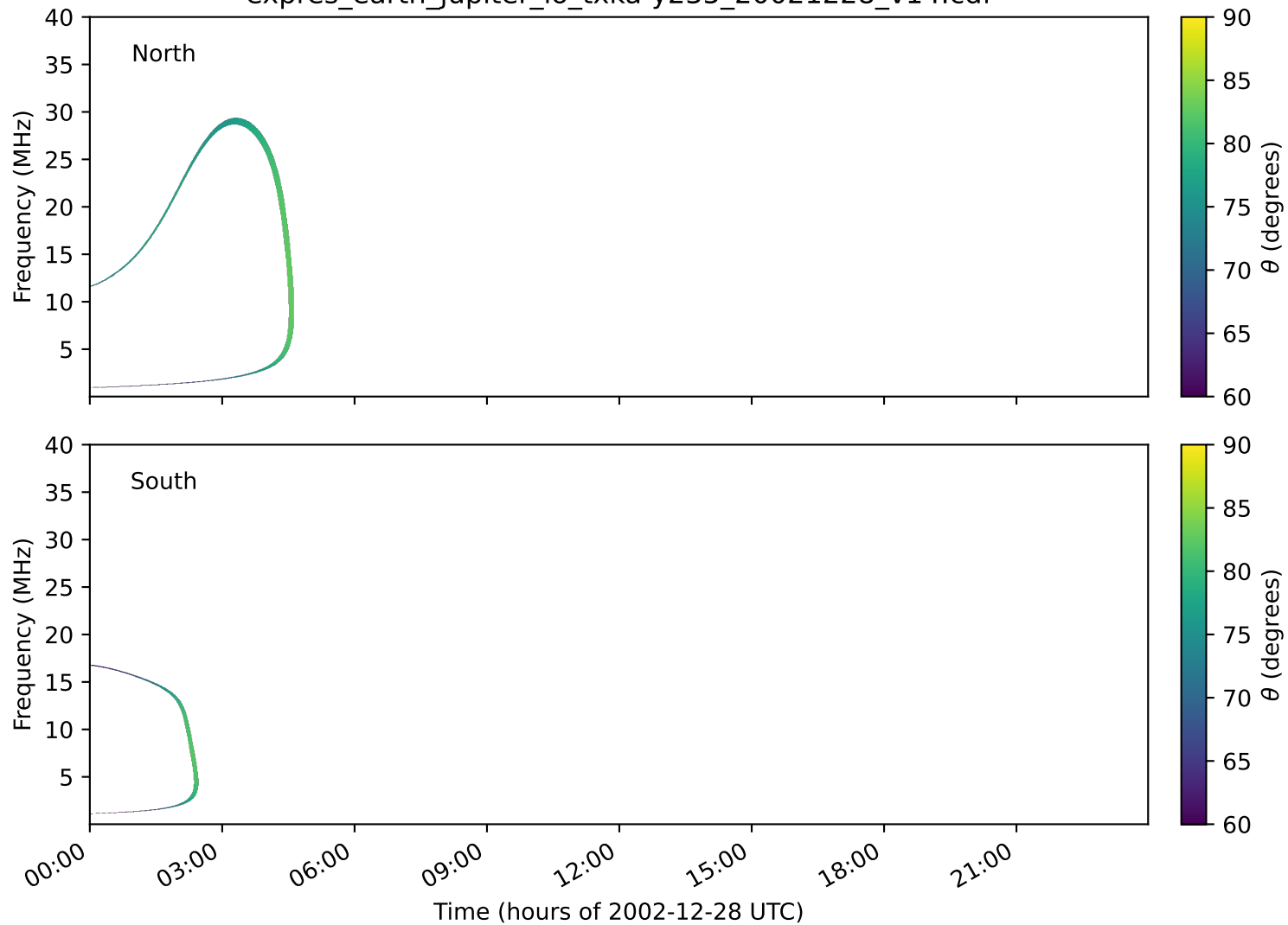
expres_earth_jupiter_io_txka-y235_20021228_v14.cdf
