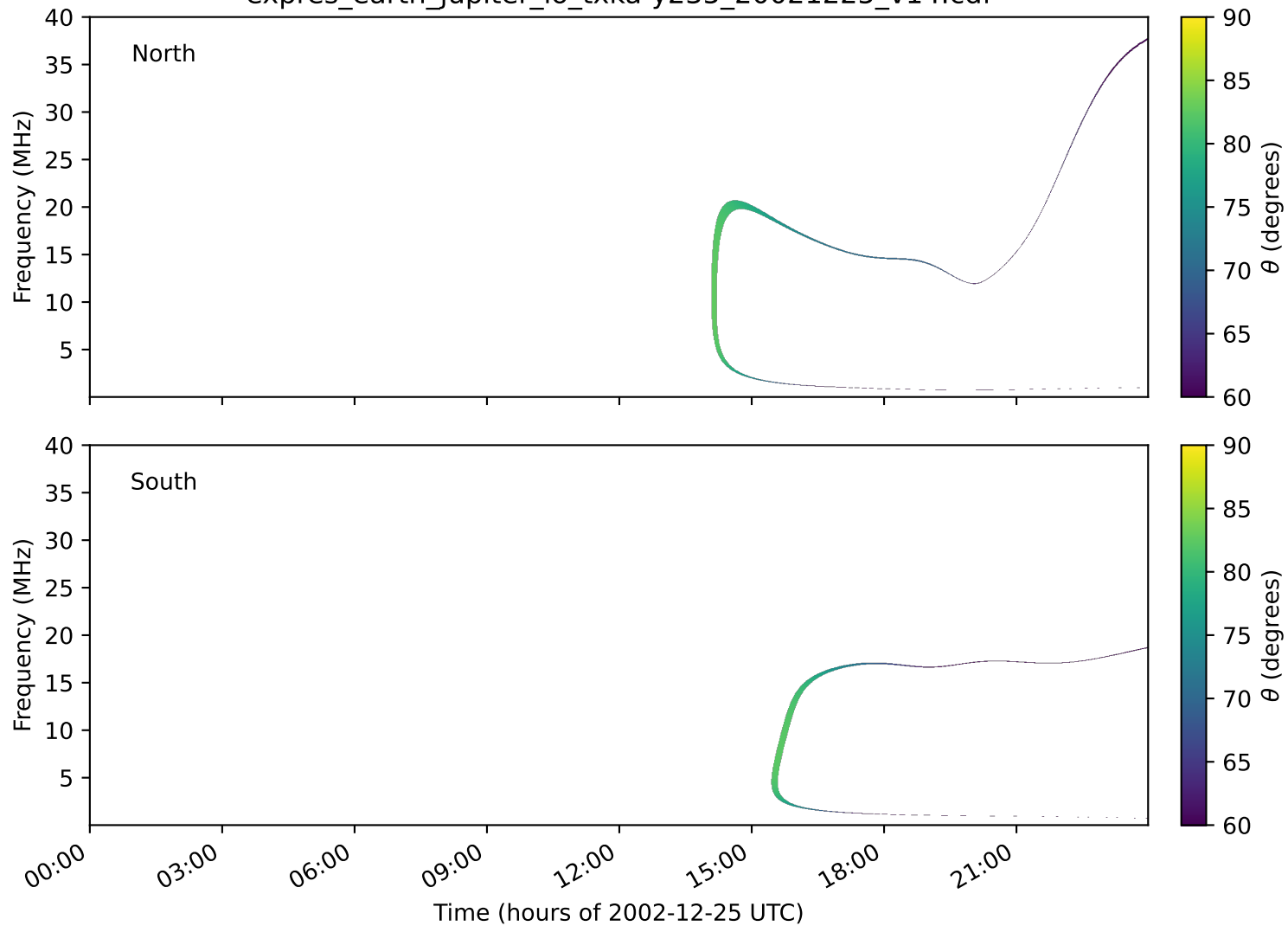
expres_earth_jupiter_io_txka-y235_20021225_v14.cdf
