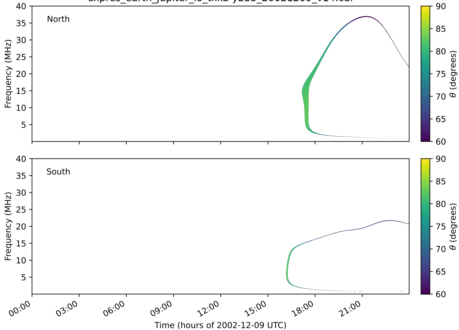
expres_earth_jupiter_io_txka-y235_20021209_v14.cdf
