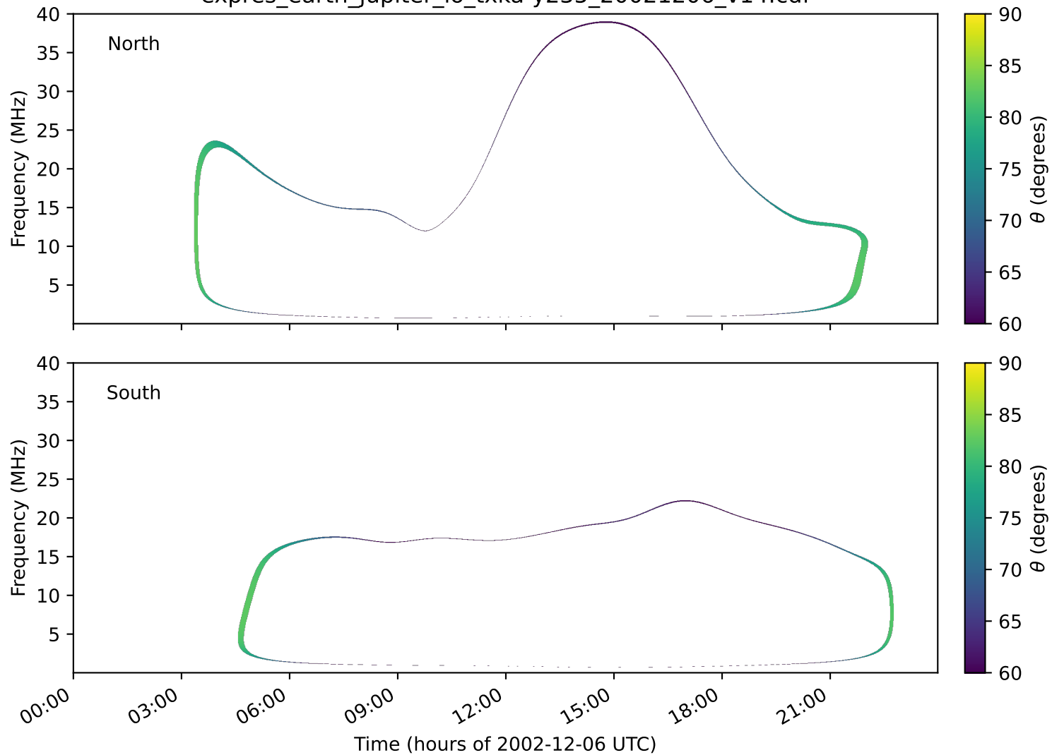
expres_earth_jupiter_io_txka-y235_20021206_v14.cdf
