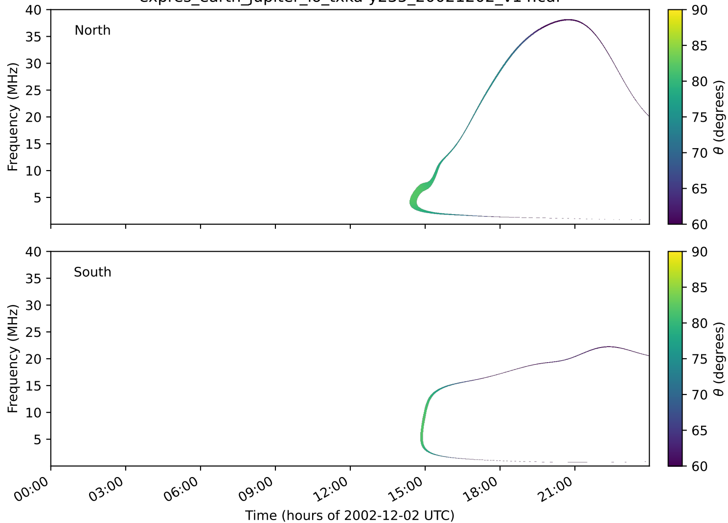
expres_earth_jupiter_io_txka-y235_20021202_v14.cdf
