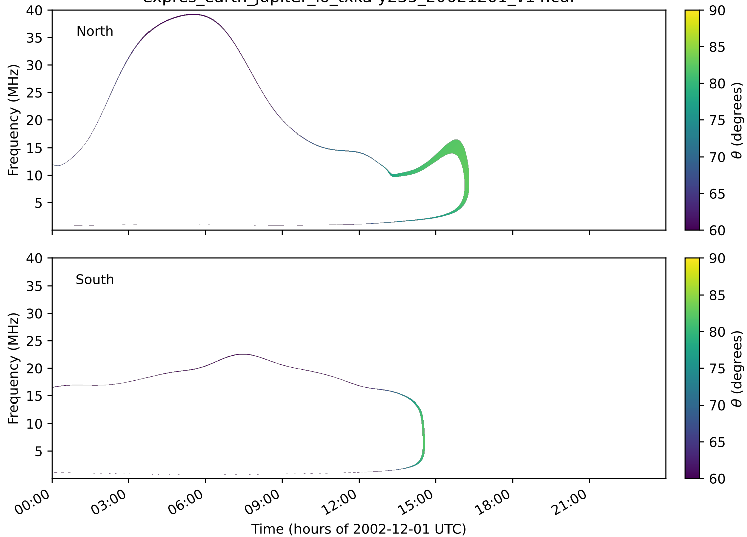
expres_earth_jupiter_io_txka-y235_20021201_v14.cdf
