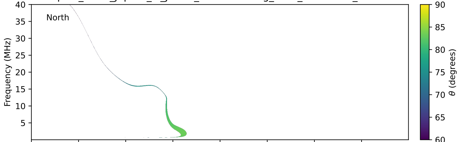
expres_earth_jupiter_io_jrm33_lossc-wid1deg_3kev_20021226_v11.cdf
