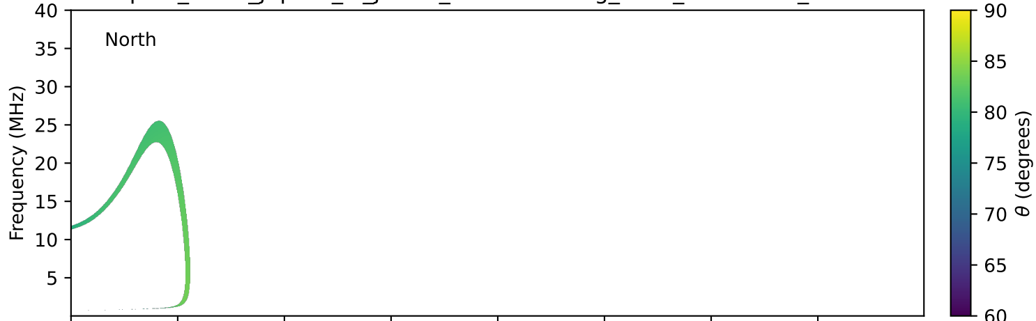
expres_earth_jupiter_io_jrm33_lossc-wid1deg_3kev_20021221_v11.cdf
