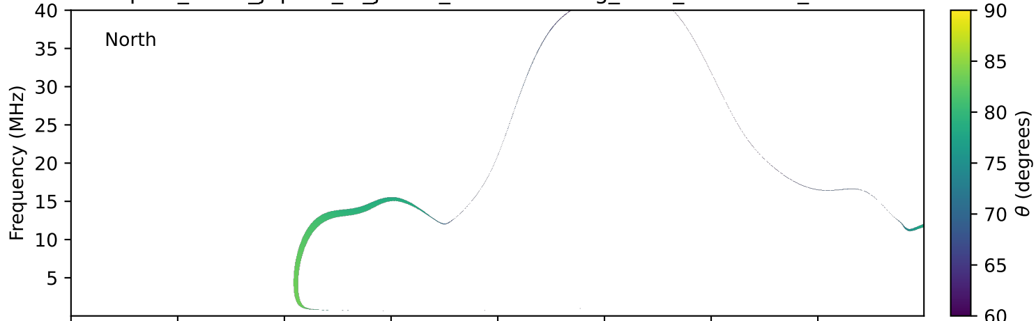
expres_earth_jupiter_io_jrm33_lossc-wid1deg_3kev_20021220_v11.cdf
