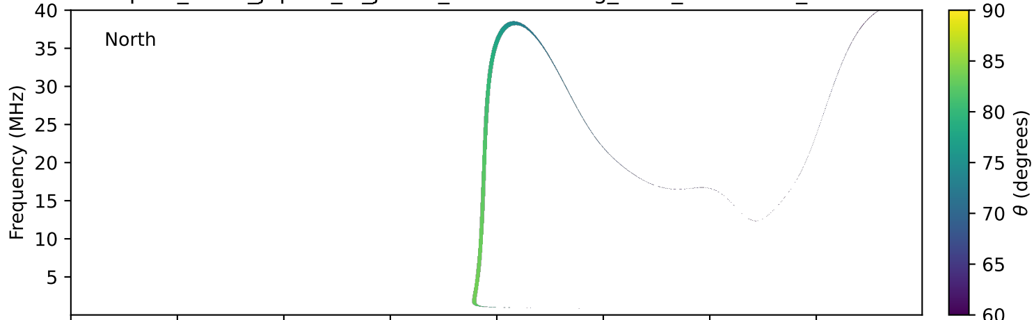
expres_earth_jupiter_io_jrm33_lossc-wid1deg_3kev_20021211_v11.cdf
