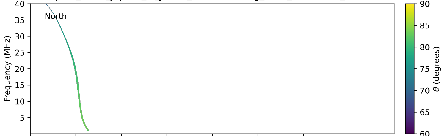
expres_earth_jupiter_io_jrm33_lossc-wid1deg_3kev_20021205_v11.cdf
